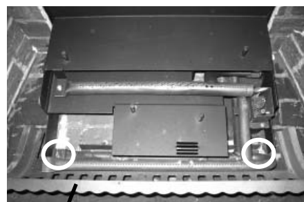
Grate
