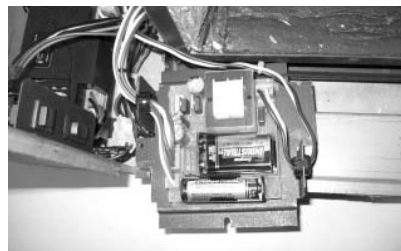
Power Module with Cover Removed
